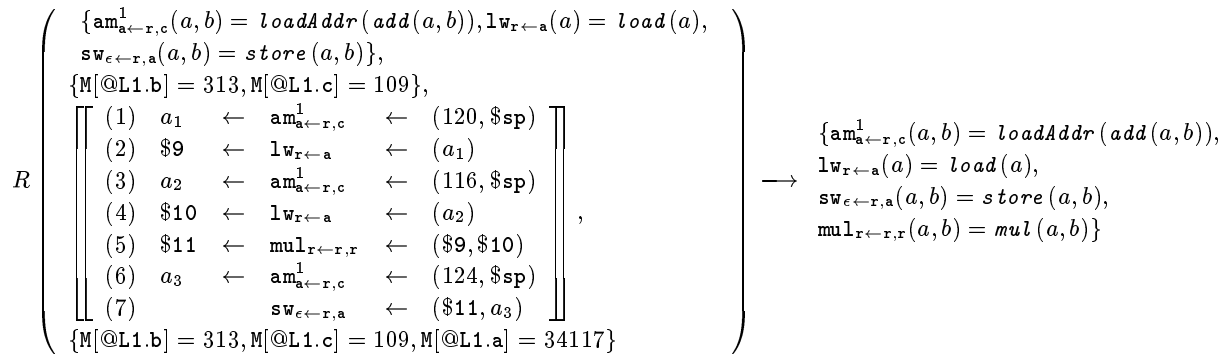
Figure 13: Reverse interpretation example. The data-flow graph in Figure 10(a) has been broken up into seven primitive instructions, each one of the form result ← operator ← (arguments) . am_{a \leftarrow r, c}^1 represents the “register+offset” addressing mode. The a_i ’s are “pseudo-registers” which hold the result of address calculations. To distinguish between instructions with the same mnemonic but different semantics (such as addl $4,%ecx and addl -8(%ebp),%edx on the x86), instructions are indexed by their signatures. lw_{r \leftarrow a} , for example, takes an address as argument and returns a result in a register.
